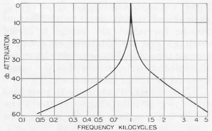
Figure 4. Selectivity curve for the 1-kc filter and Type 1231-B Amplifier. Values of second harmonic discrimination for the other filters are given in Table I, below.
