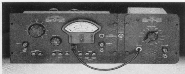
Figure 5. View of the Type 1231-P5R Filter arranged for relay-rack mounting with the Type 1231-B Amplifier and Null Detector. The filter panel attaches to the amplifier panel to make the assembly the correct width for mounting in a 19-inch relay rack. The narrow strip between the two panels carries a switch for the a-c power supply that is optional with the amplifier.
