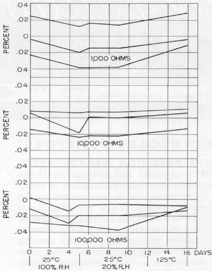
Figure 2. Measured deviations of typical resistance cards when subjected to extreme conditions of temperature and humidity. Long-term tests show a similar degree of stability.
