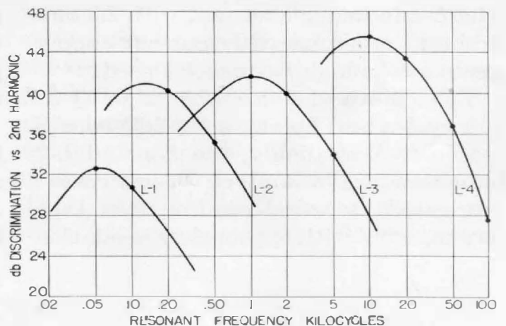
Figure 3. Low-level second harmonic discrimination versus resonant frequency for each of the four inductors.
