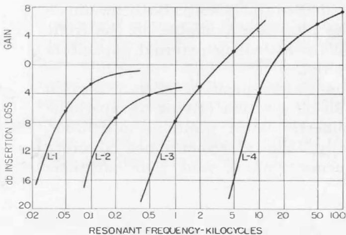
Figure 2. Low-level insertion loss versus resonant frequency for each of the four inductors.
