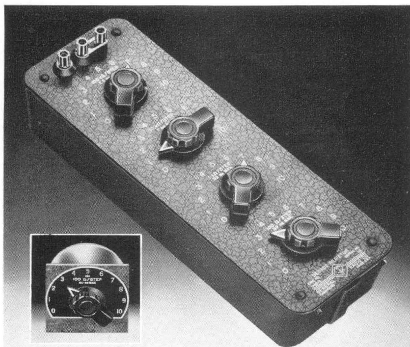
Figure 1. View of a Type 1432-A Decade Resistor. Inset at lower left shows Type 510-D Decade-Resistance Unit.
